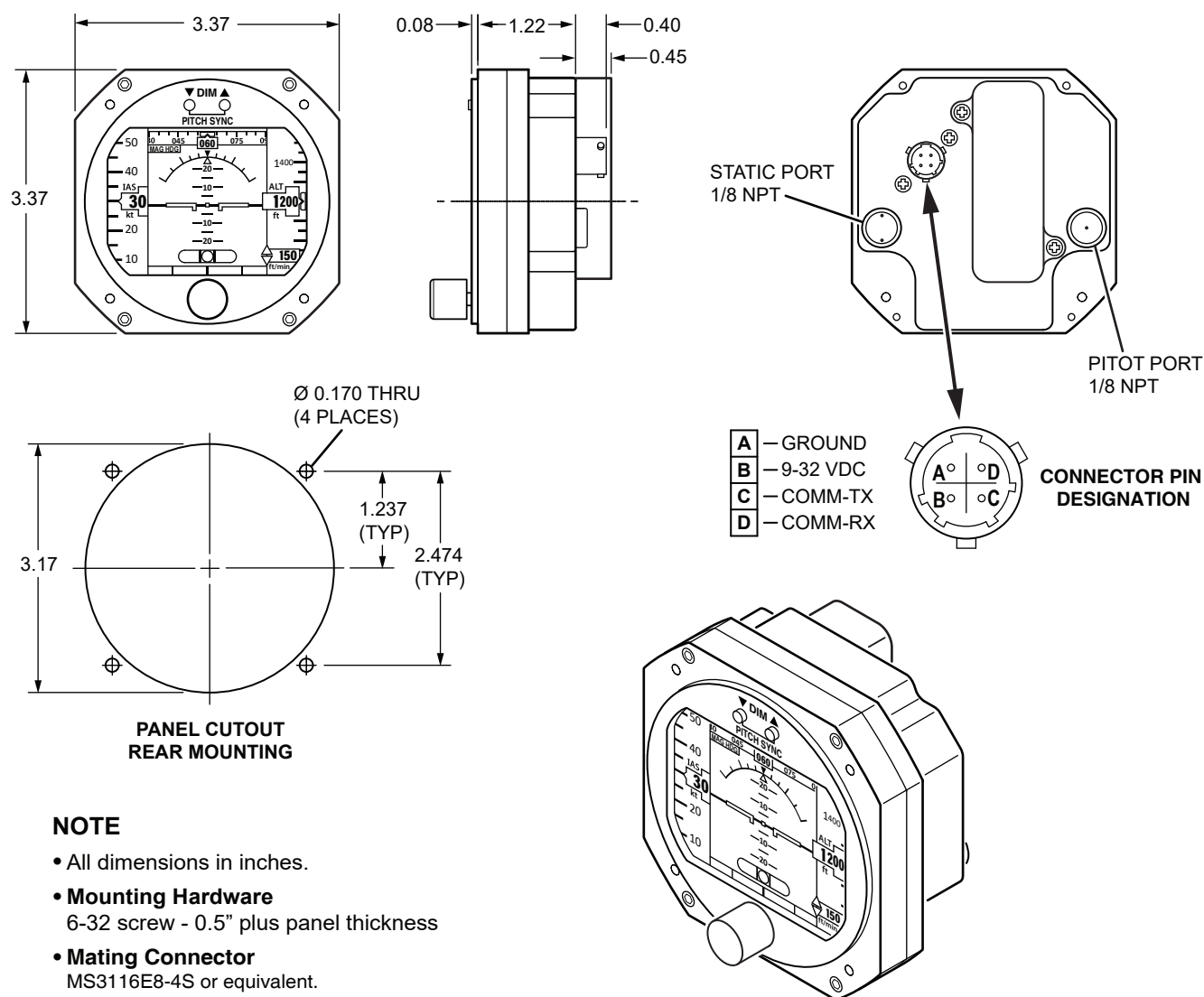
Figure 2.1, General Dimensions
